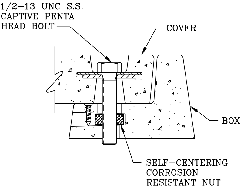
BOLT DOWN DETAIL
